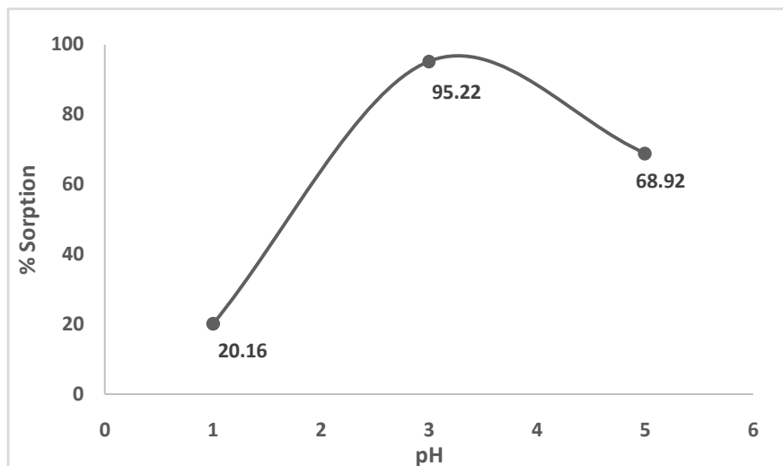
Figure 1. Percentage of Mo sorption at 200 mg L -1 at pH values of 1, 3 and 5.
